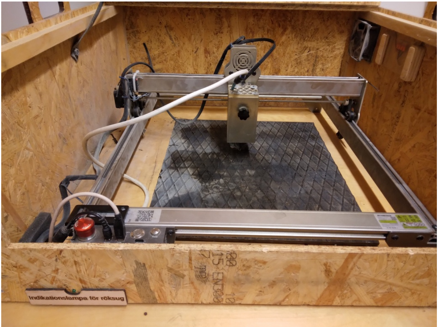
Figure 33: The opened laser cutter
